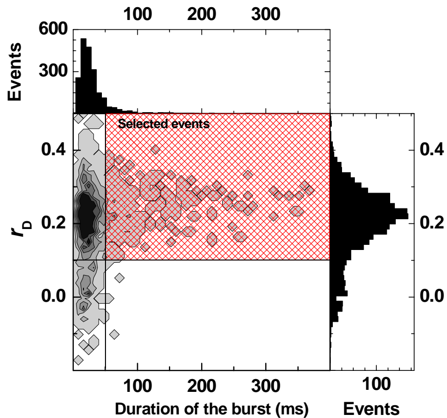
Figure I: Two-dimensional histogram of photon burst duration (i.e. diffusion time through the confocal detection volume) versus anisotropy r_D of the donor fluorophore (rhodamine 110) attached to the \gamma -subunit of F_0F_1 -ATP synthase during ATP hydrolysis. The events resulting from the FRET-labeled holoenzyme incorporated in a liposome can be distinguished from unbound dye and remaining donor labeled F_1 parts (not bound to F_0 ) by their high r_D . The probability to observe a transition between two FRET levels within a photon burst depends on the duration of the event. Therefore, only photon bursts within the red shaded area are considered for further analysis (i.e. 382 bursts of 2127 bursts with r_D > 0.12 ).
