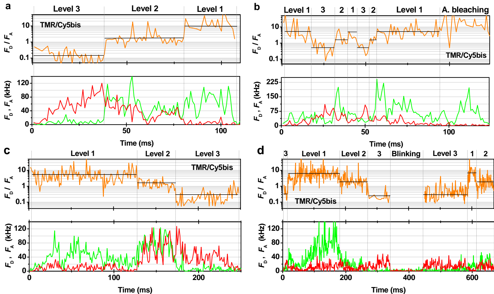
Figure II: Photon bursts of single FRET-labeled F_0F_1 -ATP synthases in liposomes during ATP hydrolysis ( a , b ), and during ATP synthesis ( c , d ). FRET donor is TMR, FRET acceptor is Cy5bis in all traces. Corrected fluorescence intensity traces of the donor, F_D , and acceptor, F_A , are shown in green and red, respectively, corrected intensity ratios F_D/F_A are depicted in orange with a time window of 1 ms. Three distinct FRET levels are attributed (1, 2 or 3) at the top of the figures. Black horizontal lines indicate the mean FRET levels taken from the histogram, vertical lines mark beginning and end of a level. In trace ( b ), the enzyme exhibits short dwell times for a FRET level, i.e. fast ATP turnover is depicted. In trace ( d ), photophysical fluorophore blinking after 340 ms interrupts the detection of FRET states for approximately 100 ms before ongoing ATP synthesis is demonstrated by interchanging FRET levels.
